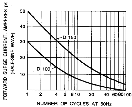
Fig. 1 - MAXIMUM NON-REPETITIVE SURGE CURRENT
