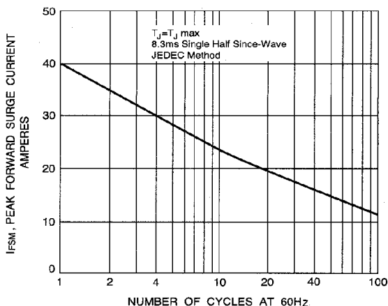
FIG.5-MAXIMUM NON-REPETITIVE PEAK FOWARD SURGE CURRENT
