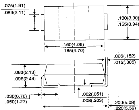
SMB/DO-214AA
