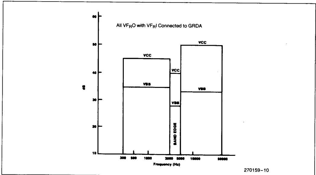
Figure 10. Receive Filter
