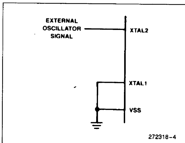
Figure 4. External Drive Configuration
