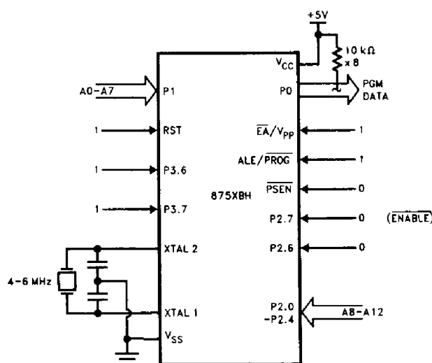
Figure 10. Verifying the EPROM
