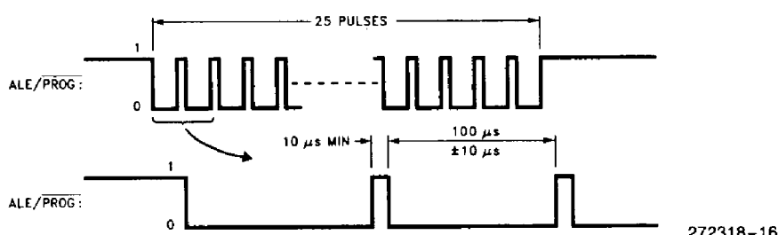
Figure 9. PROG Waveforms
