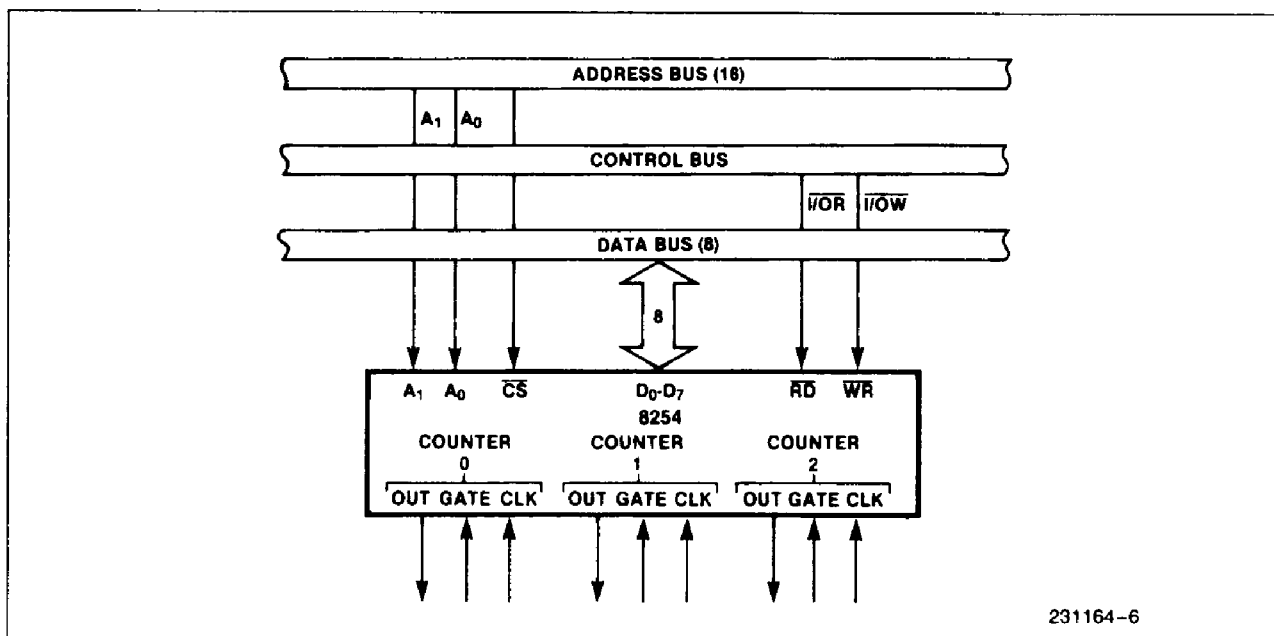
Figure 6. 8254 System Interface
