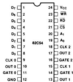
Diagrams are for pin reference only. Package sizes are not to scale. Figure 2. 82C54 Pinout
