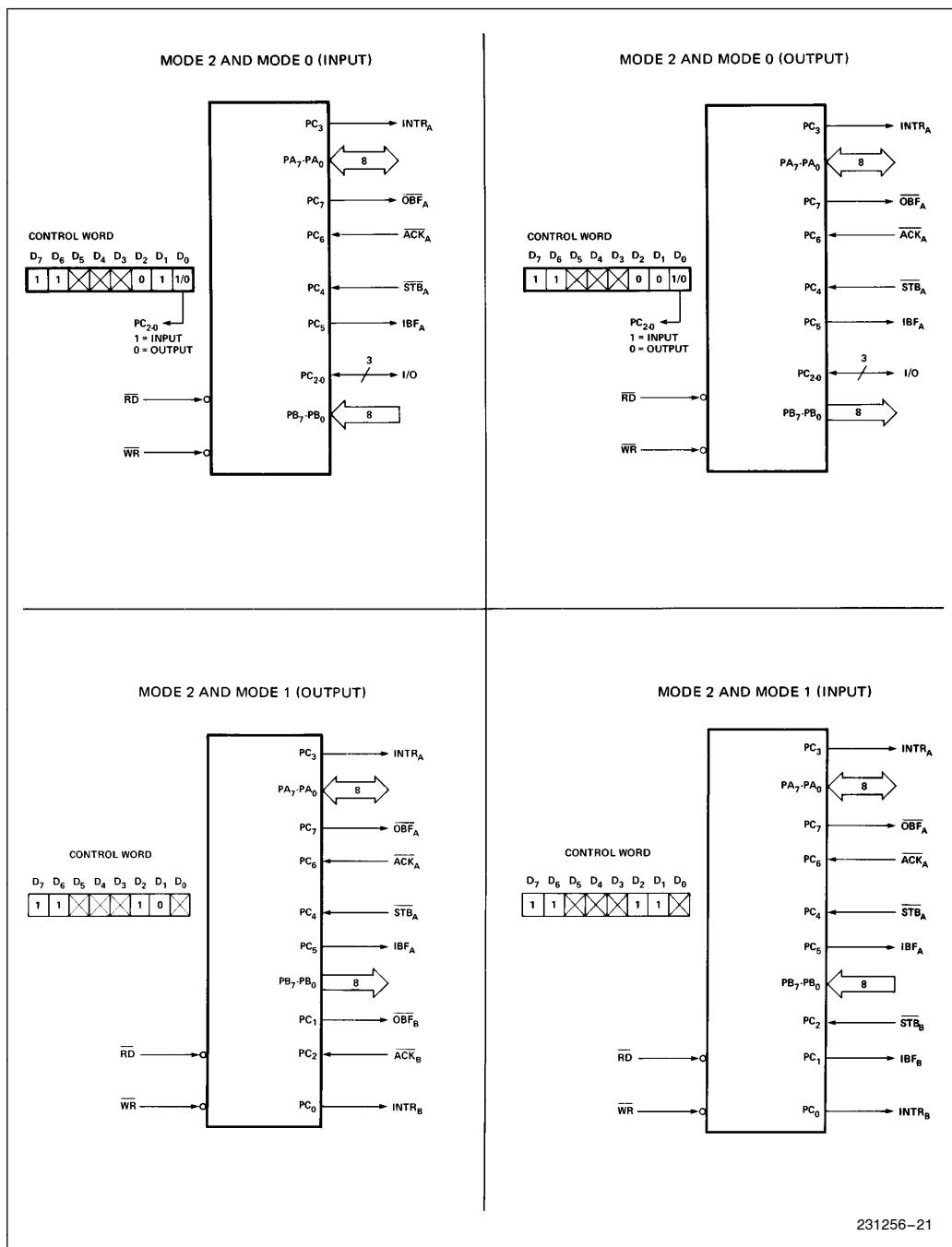
Figure 16. MODE 1/4 Combinations
