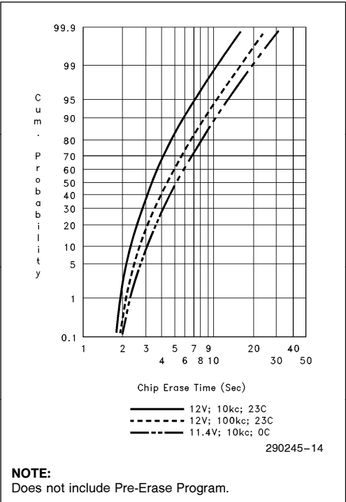
Figure 10. 28F020 Typical Erase Capability
