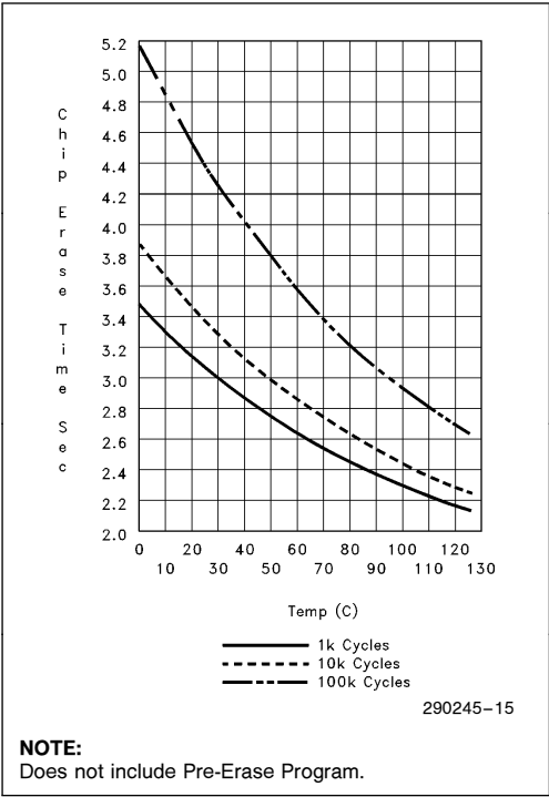
Figure 11. 28F020 Typical Erase Time at 12.0V
