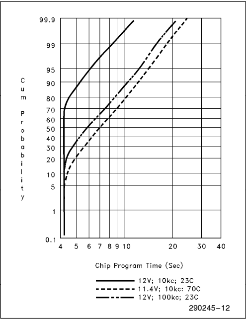
Figure 8. 28F020 Typical Programming Capability
