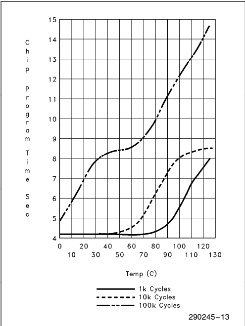
Figure 9. 28F020 Typical Program Time at 12V
