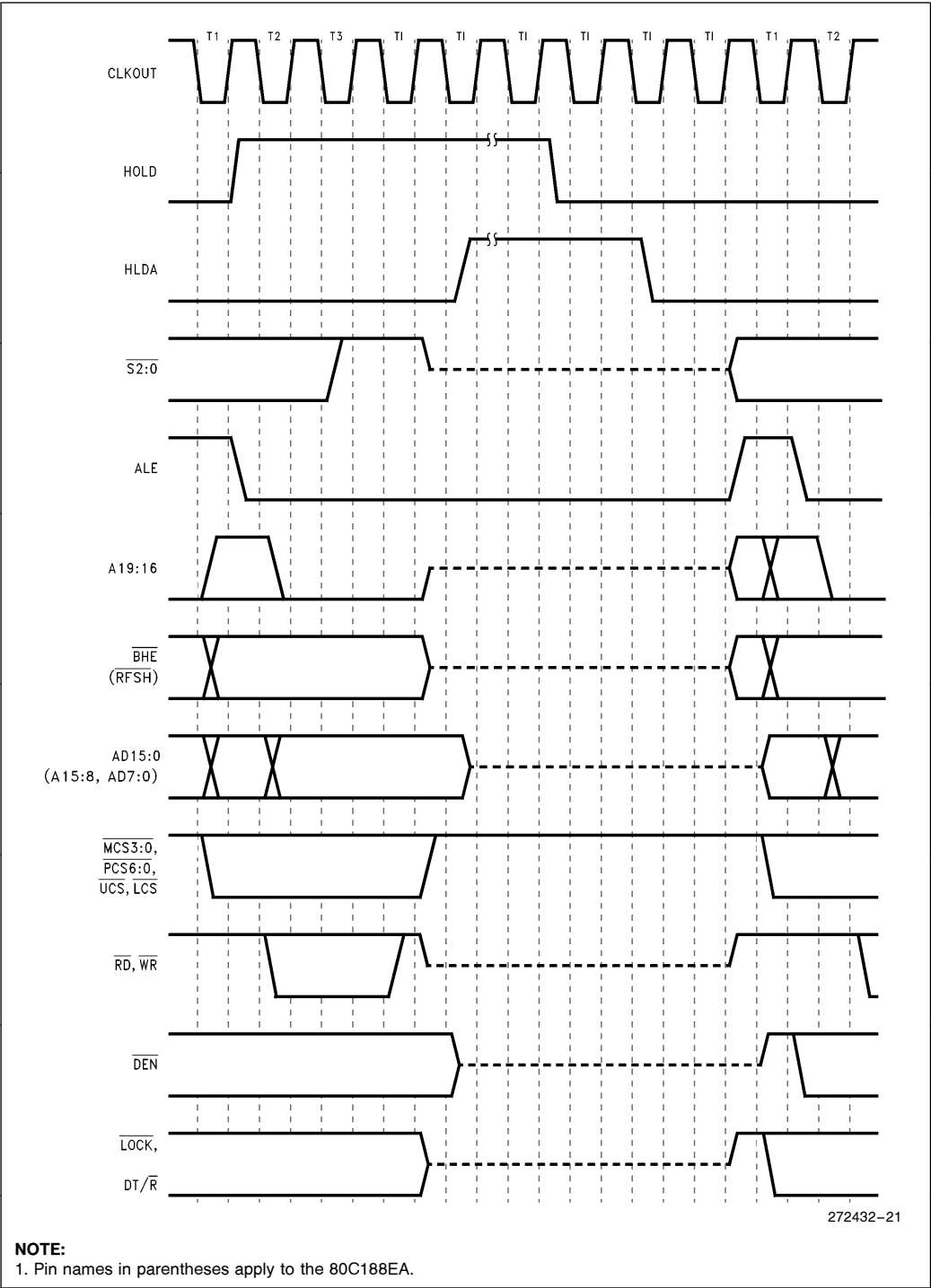
Figure 21. HOLD/HLDA Waveform
