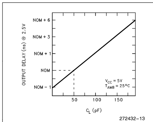
Figure 13. Typical Output Delay Variations Versus Load Capacitance
