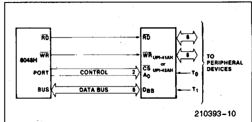
Figure 6. 8048H-UPI-41/42 Interface
