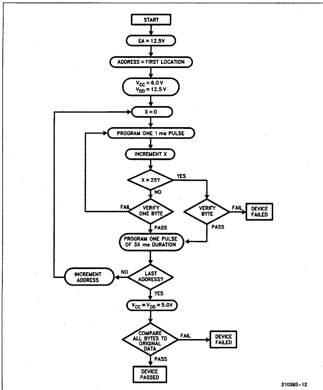
Figure 9. Programming Algorithm
