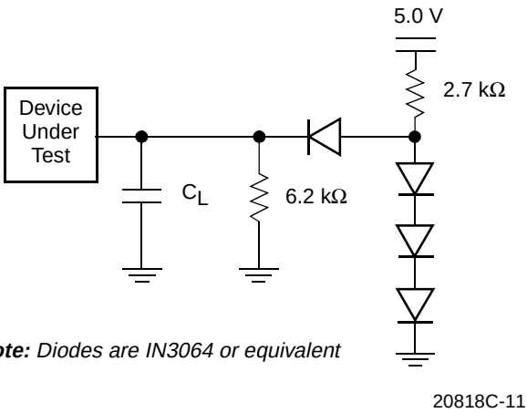
Figure 8. Test Setup
