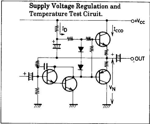
Test Circuit
