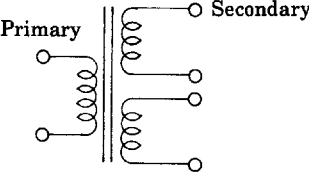
Data on transformer (T1)
