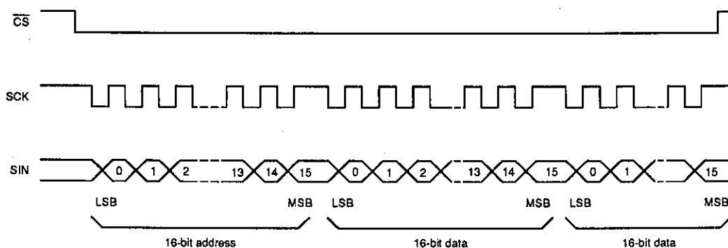
Figure 1. Input timing
