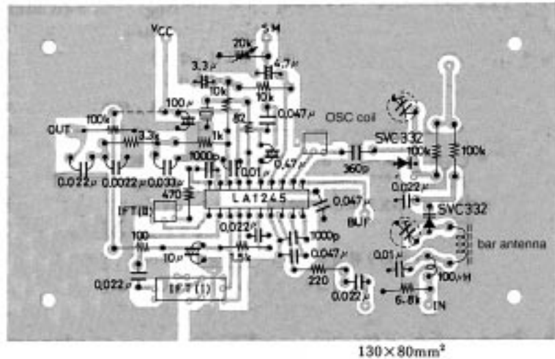
An Example of Printed Pattern (130×80mm 2 , bottom view)
