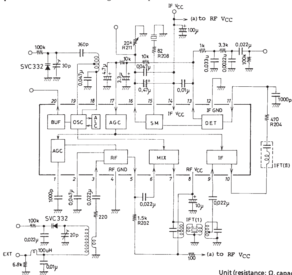
Sample Application Circuit 2 : Using variable capacitance diodes
