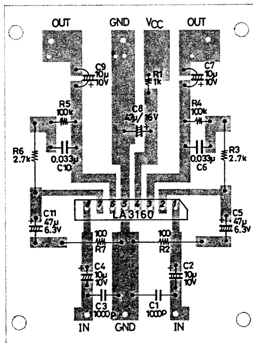
Sample Printed Circuit Pattern (Cu-foiled area, 67×50mm 2 )
