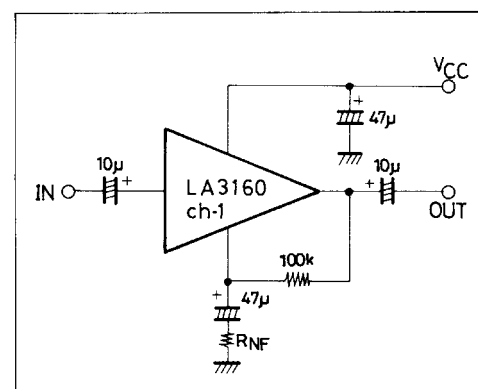
Test Circuit 2
