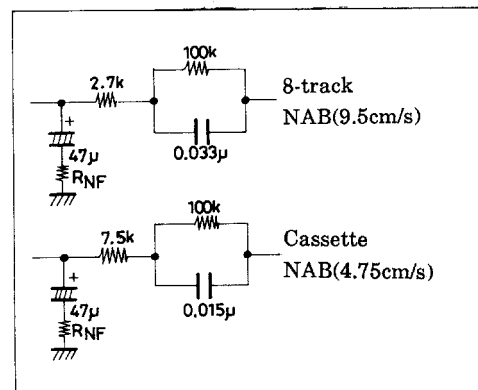
Test Circuit 1
