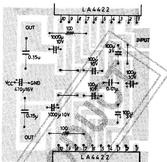
Sample Printed Circuit Pattern (45 x 43mm 3 , Cu-foiled side)
