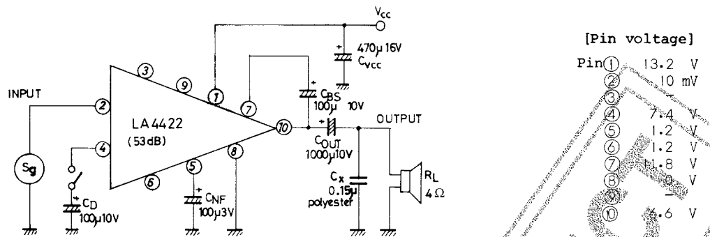
Sample Application Circuit 1. Power amplifier for 5.8W typ. car radio, car stereo
