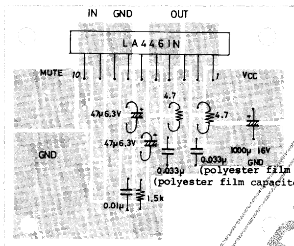
Sample Printed Circuit Pattern of LA4461N (Cu-foiled side) 40 x 50mm 2
