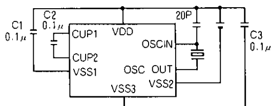
Fig. 9 Supply Current, Oscillation Hold Voltage Test Circuit
