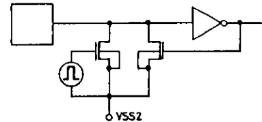
Fig. 4 S1-4, M1-4 Input Configuration
