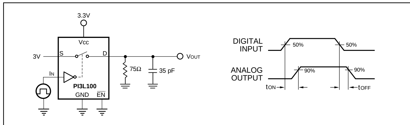
Figure 1. Switching Time
