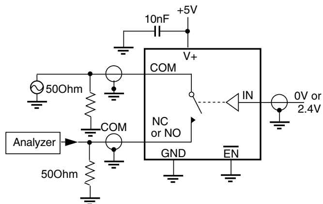
Figure 3. Off Isolation
