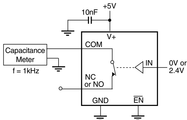
Figure 6. Channel-On Capacitance
