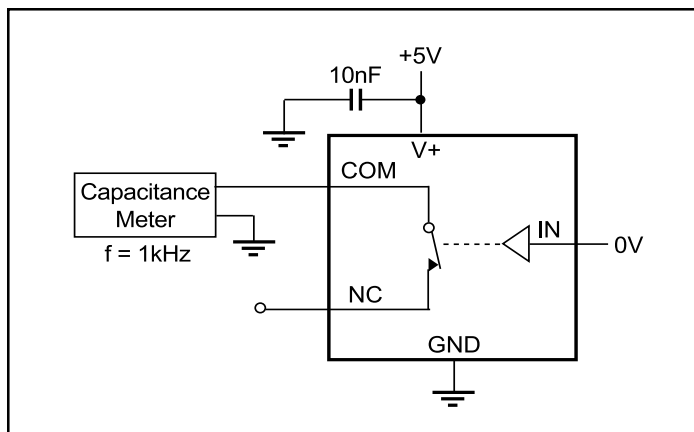
Figure 6. Channel-On Capacitance
