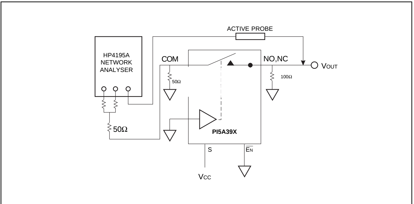
Figure 5. Off Isolation
