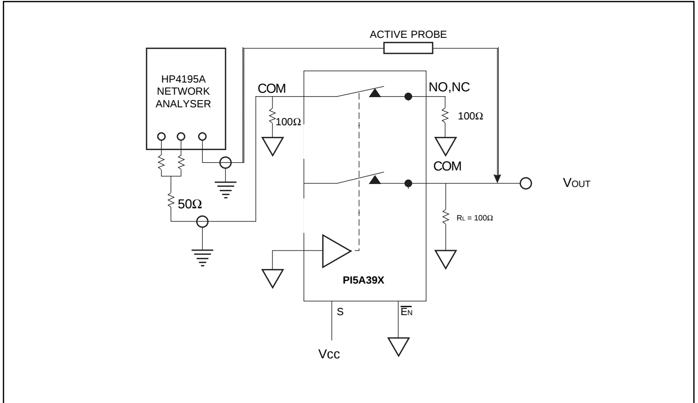
Figure 4. Crosstalk
