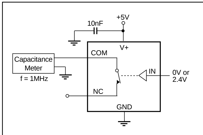
Figure 7. Channel-On Capacitance
