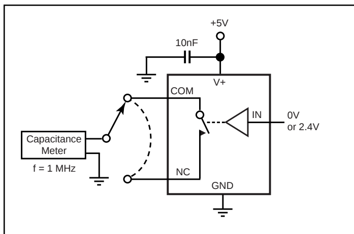
Figure 6. Channel-Off Capacitance
