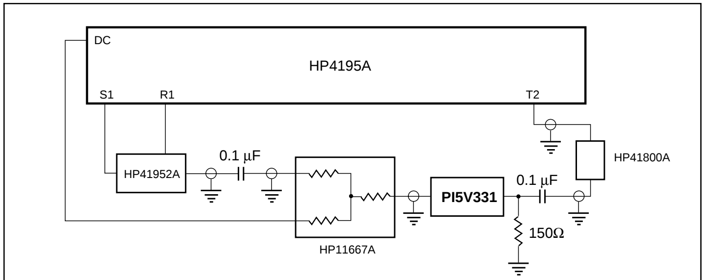
Figure 1. Differential Gain/Phase
