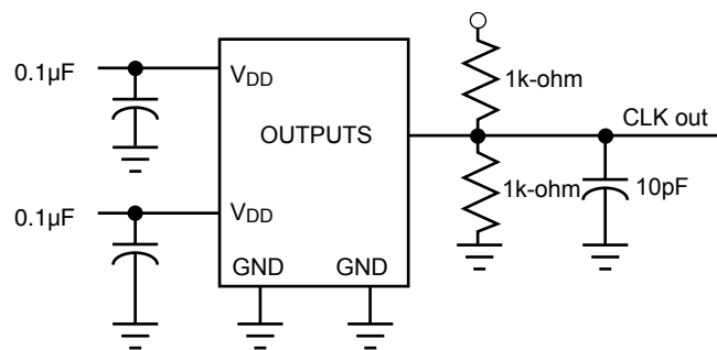
Test Circuit 2
