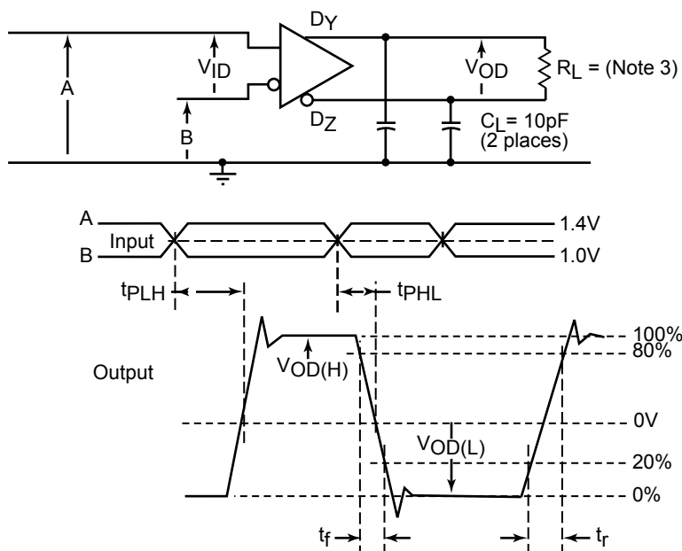
Figure 6. Test Circuit and Definitions
