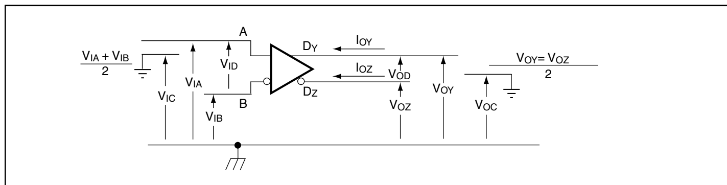
Figure 4. Voltage Definitions
