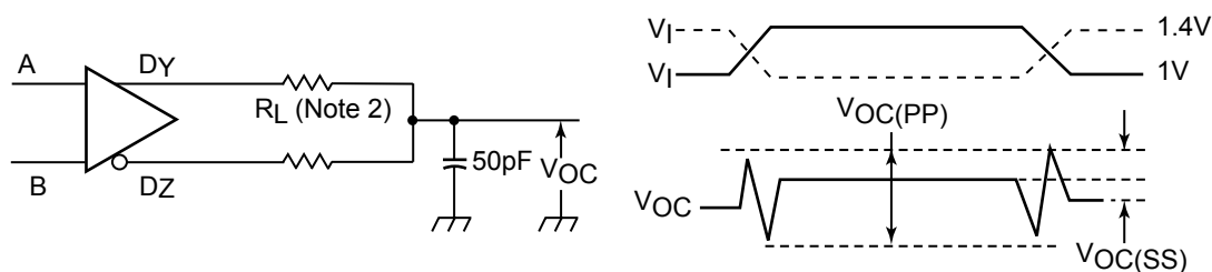
Figure 5. Test Circuit and Definitions for the Driver Common-Mode Output Voltage
