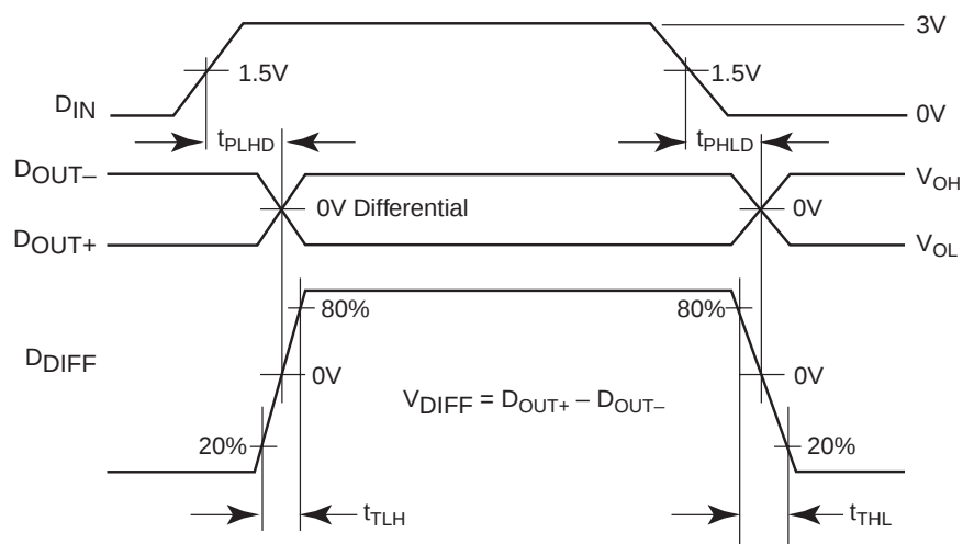
Figure 3. Driver Propagation Delay and Transition Time Waveforms
