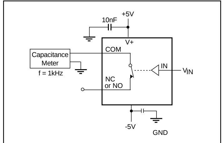
Figure 8. Channel-On Capacitance
