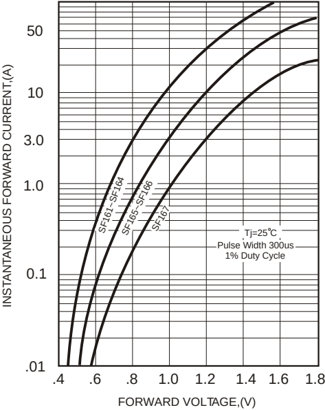
FIG.3-TYPICAL FORWARD CHARACTERISTICS
