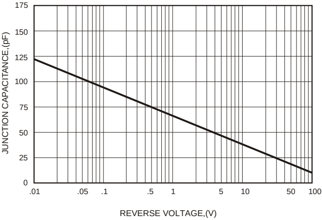
FIG.6-TYPICAL JUNCTION CAPACITANCE
