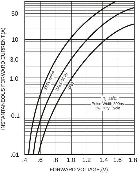
FIG.3-TYPICAL FORWARD CHARACTERISTICS
