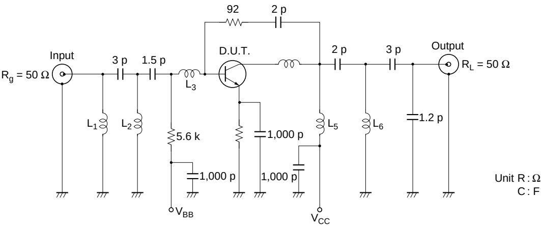
Circuit Example-UHF Wide Bandwidth Amplifier (f = 500 MHz to 950 MHz)
