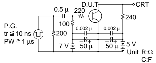
Switching Time Test Circuit t_{stg} Test Circuit
