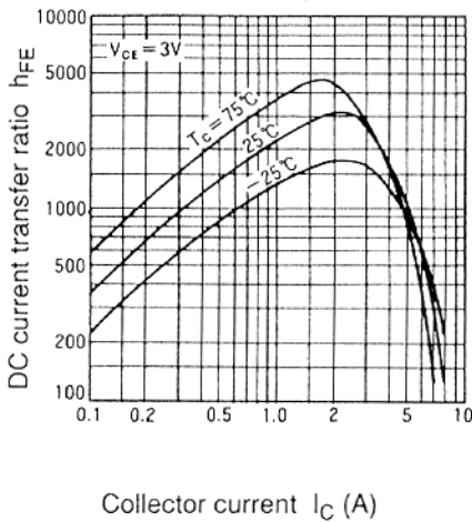
DC Current Transfer Ratio vs. Collector Current
