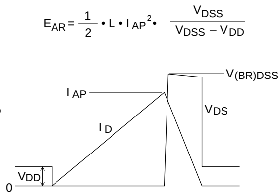
Avalanche Waveform
