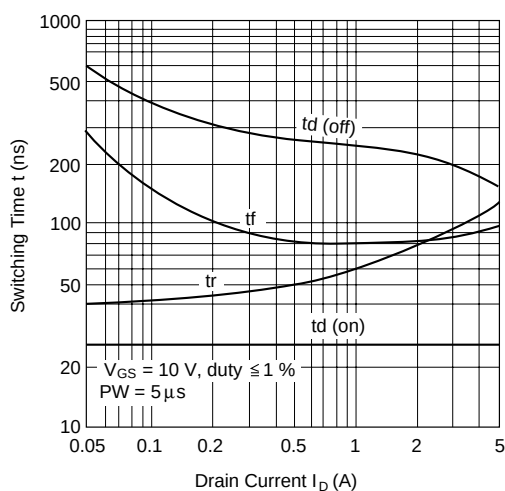
Switching Characteristics
