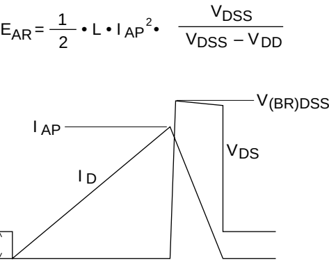
Avalanche Waveform
