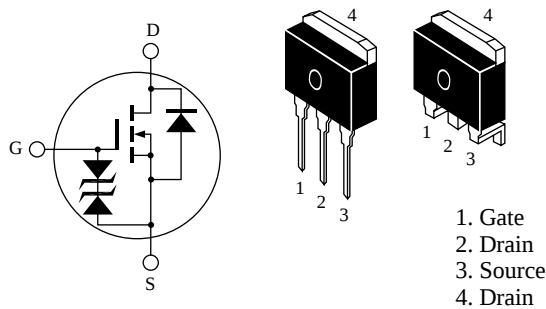
LDBPAK
