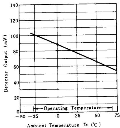
DETECTOR OUTPUT vs. AMBIENT TEMPERATURE
