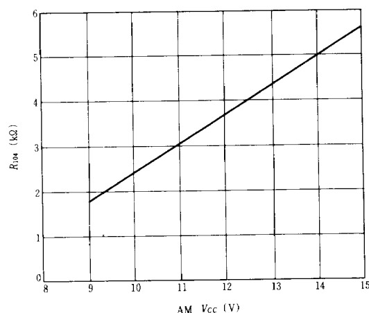
■ R_{104} (Resistor of Pin-15) vs. AM V_{cc}
