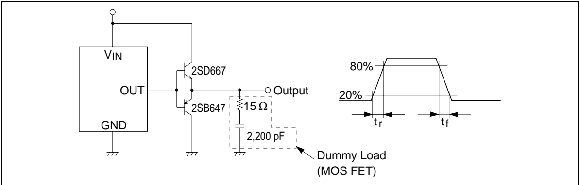
Figure 5 t r • t f Measurement Circuit
