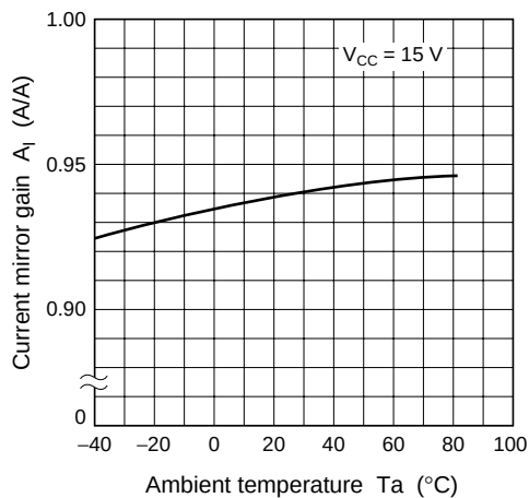
Current Mirror Gain vs Ambient Temperature
