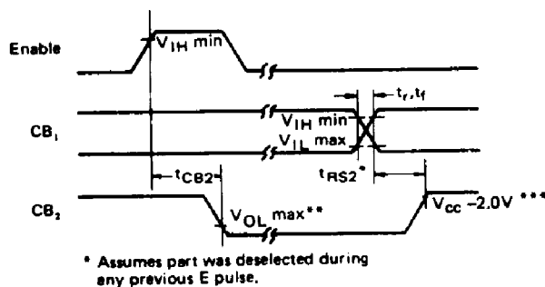
Figure 7 CB 2 Delay Time (Write Mode; CRB5=1, CRB3=CRB4=0)
