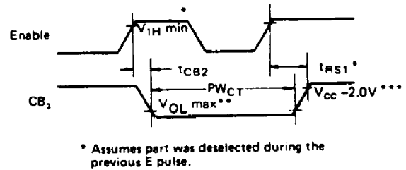
Figure 6 CB 2 Delay Time (Write Mode; CRB5=CRB3=1, CRB4=0)
