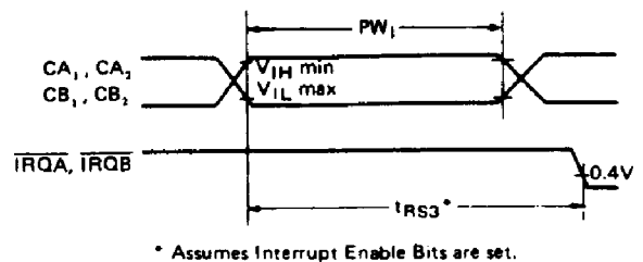
Figure 8 Interrupt Pulse Width and \overline{IRQ} Response
