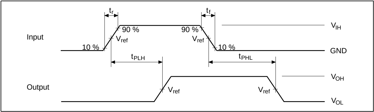
Waveforms – 2
