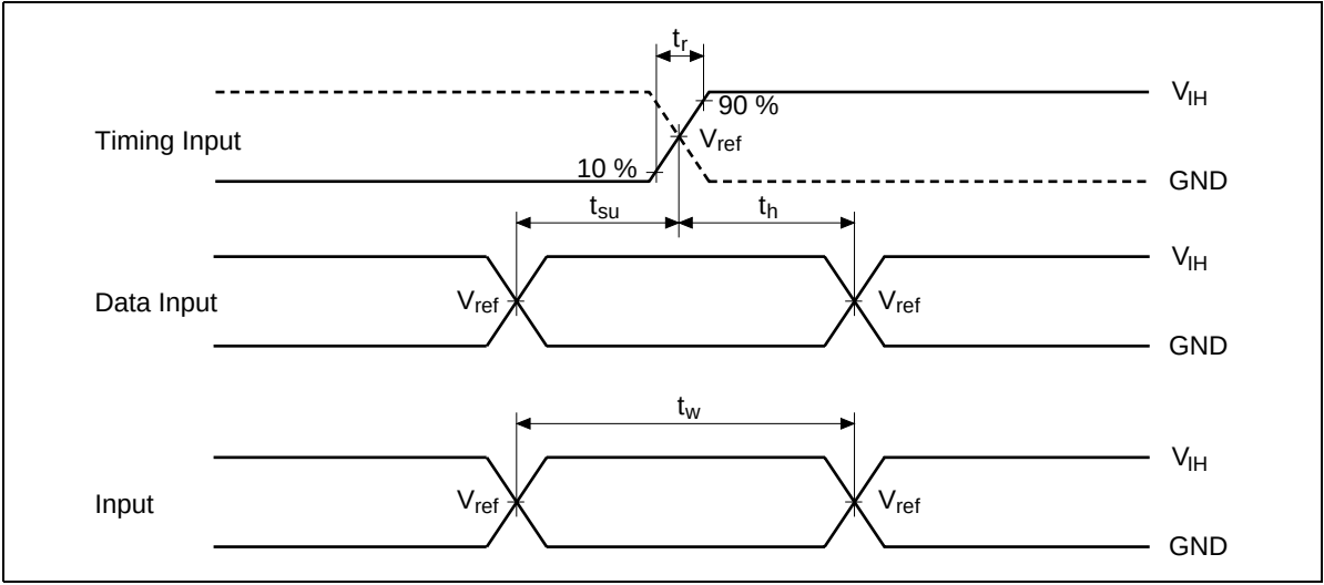
Waveforms – 2
