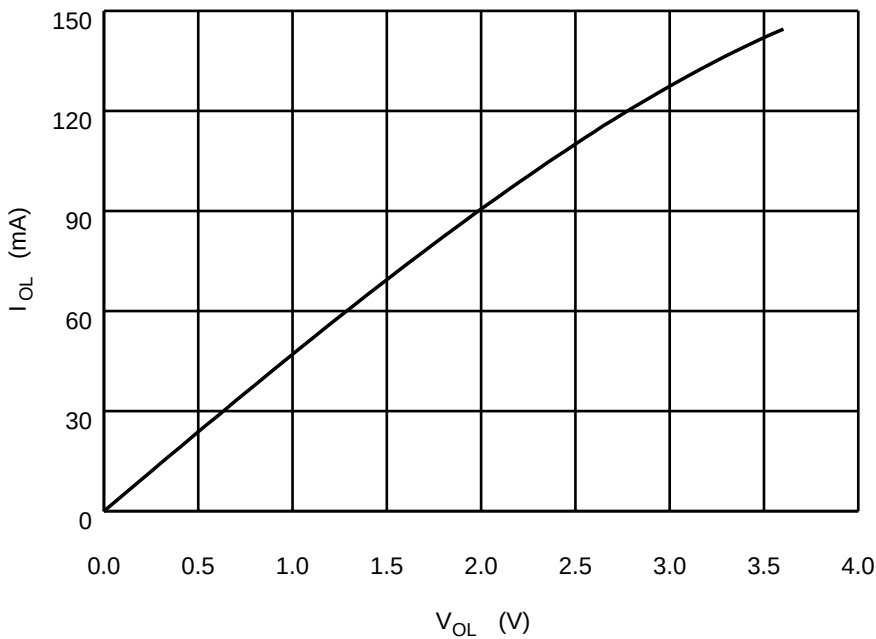
Strong condition LOW V_{CC} = 3.6\text{ V} , T_a = 0^\circ\text{C}
