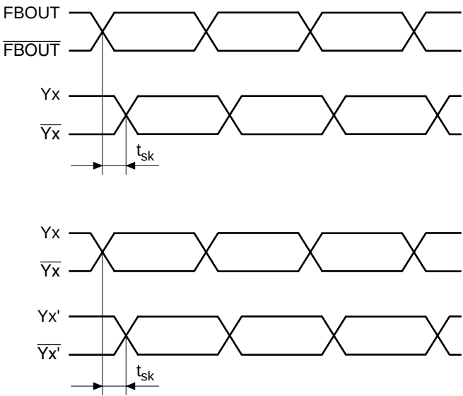
Figure 4 Output skew
