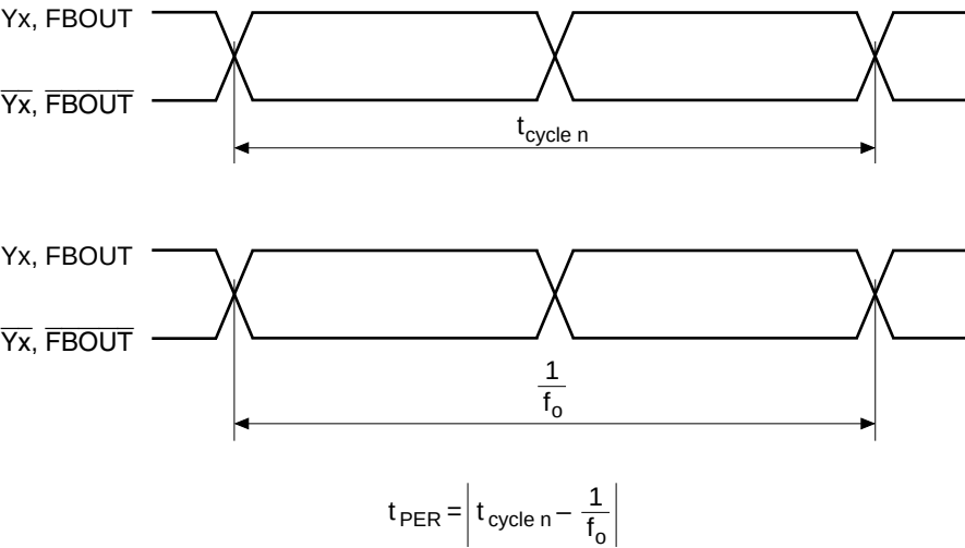
Figure 6 Period jitter
