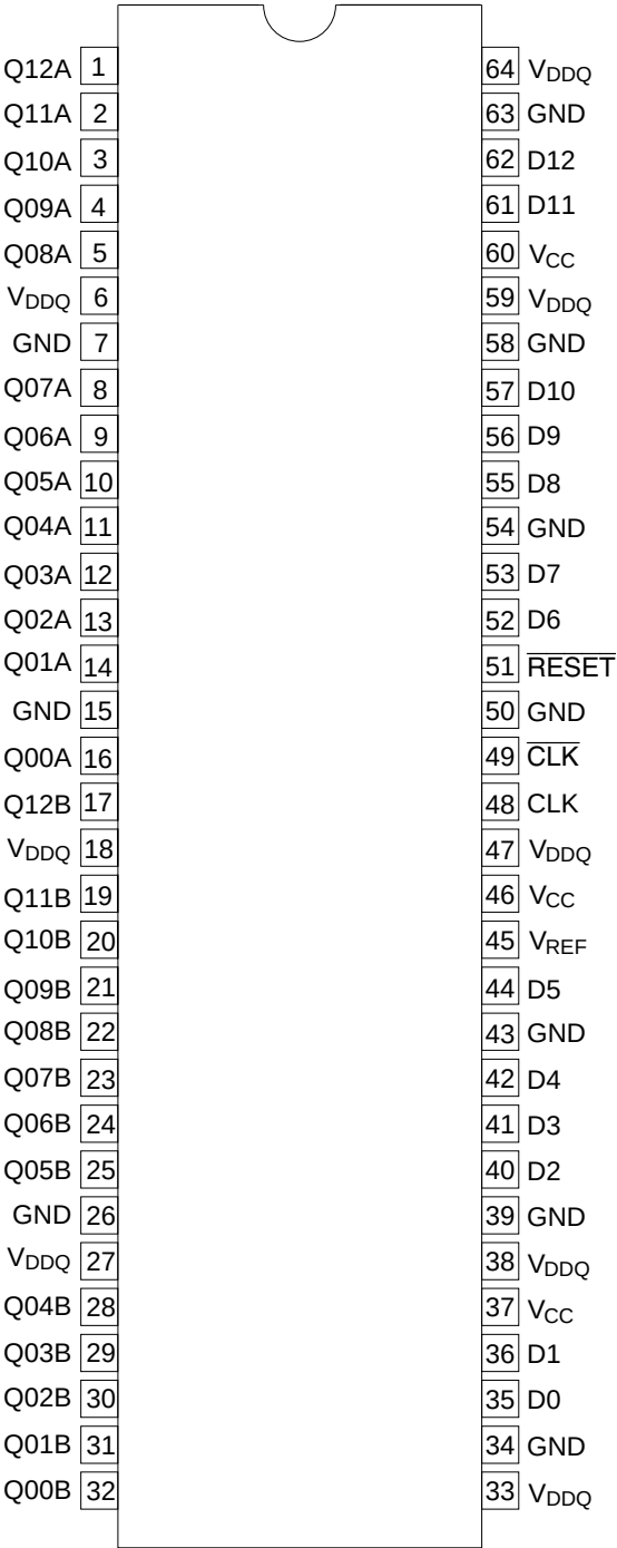
(Top view)
