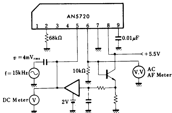
Test Circuit 3 (G V )
