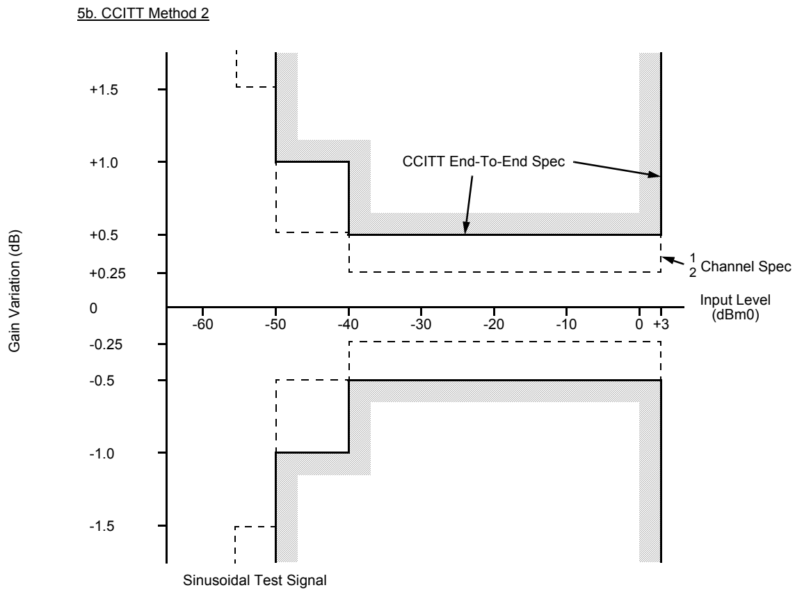
Figure 12 - Variation of Gain With Input Level
